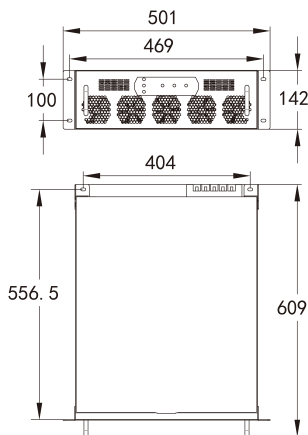
30-50kvar Rack-mounted type
