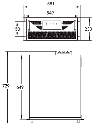
75-100kvar Rack-mounted type
